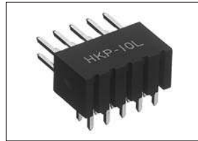
Right-angle through hole type male connector for PCB HKP-( )M6L D-18 HKP series...16
