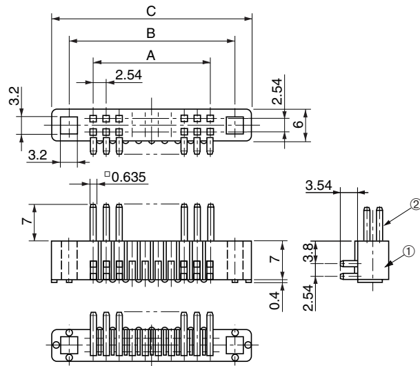
Right-angle type HKP-( )M4L
