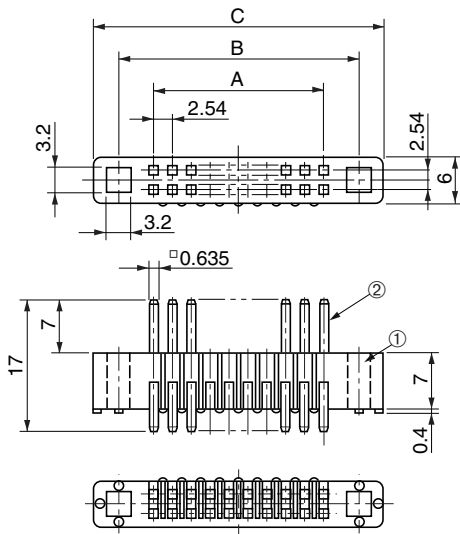
Straight type HKP-( )M4
