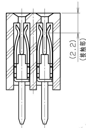
X-X' 断面 (5/1) X-X' SECTION
