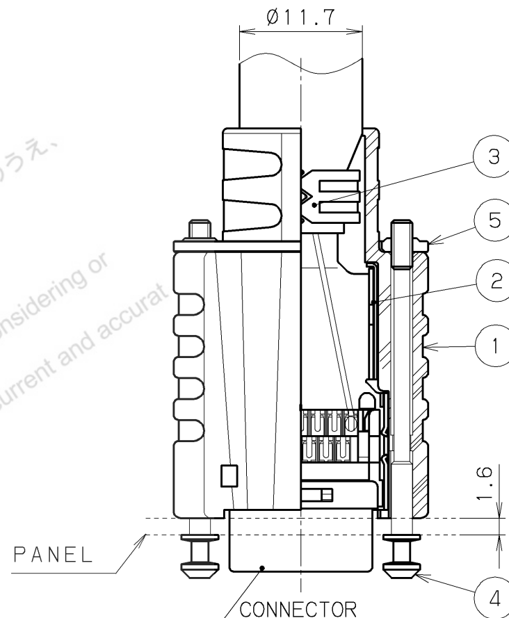
HDR-E26FSG1+ AFTER ASSEMBLY DRAWING
