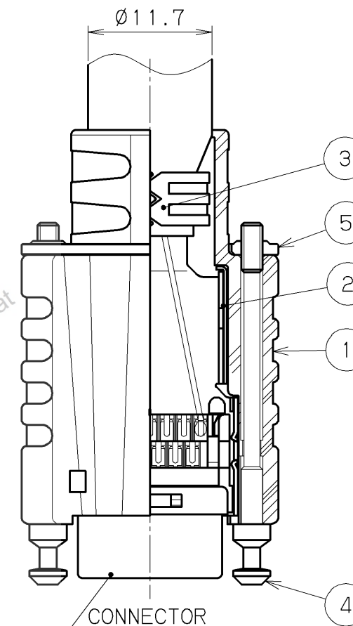
CONNECTOR HDR-E26FSG1+ AFTER ASSEMBLY DRAWING
