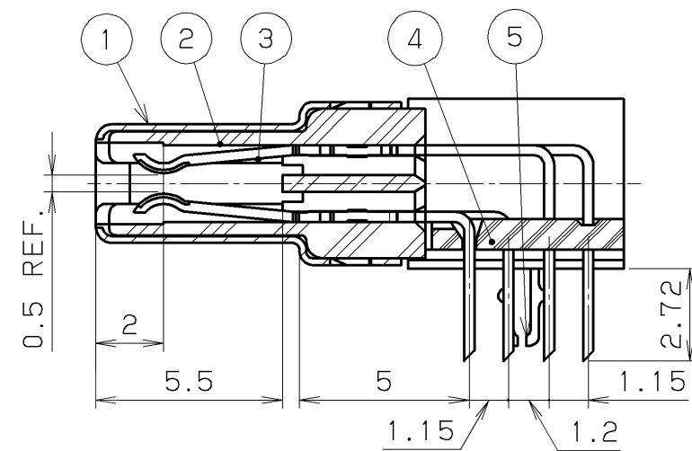
CONTACT DETAIL
