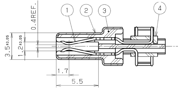
CONTACT DETAIL (5/1)
