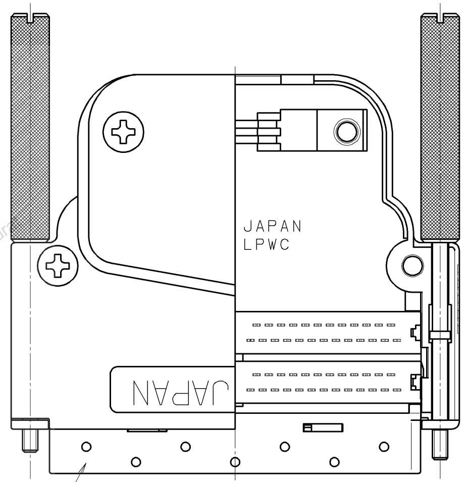
CONNECTOR P/N: HDRA-E100M ( ) 1 DRAWING AFTER CONNECTOR ASSEMBLY
