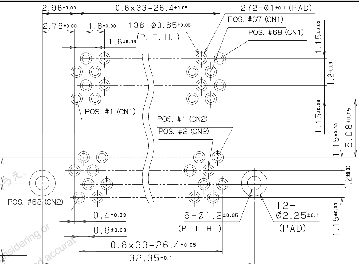
RECOMMENDED P. C. B. LAYOUT t=1.6±0.1 (SCALE=5/1) MOUNT SIDE VIEW
