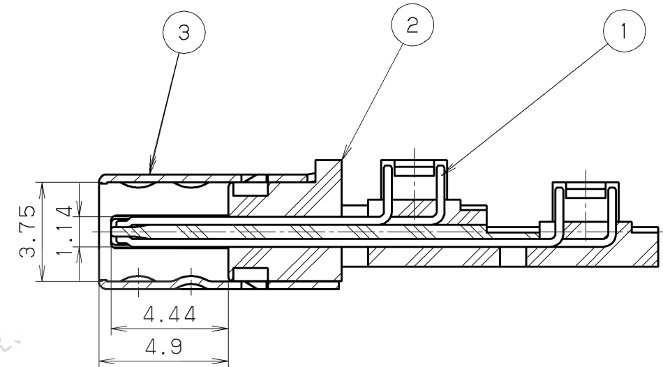
CONTACT DETAIL (5/1)
