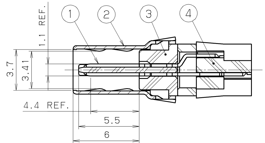
CONTACT DETAIL (S=5/1)
