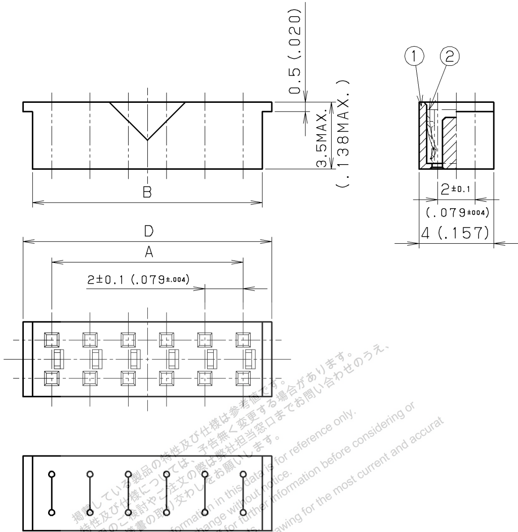
DETAIL FIGURE SHORT CIRCUIT
