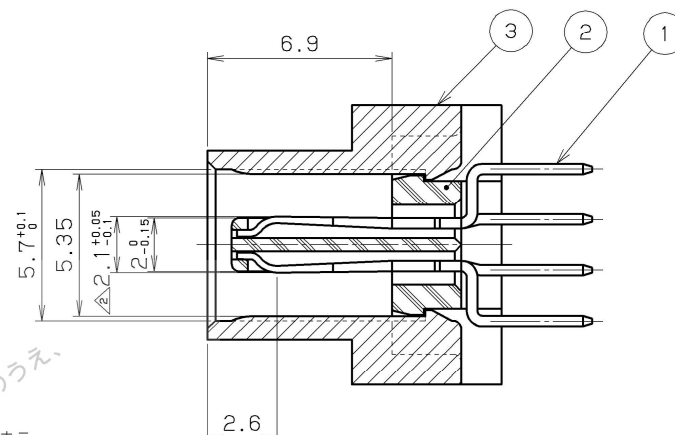
X-X 断面矢視 (5/1)
