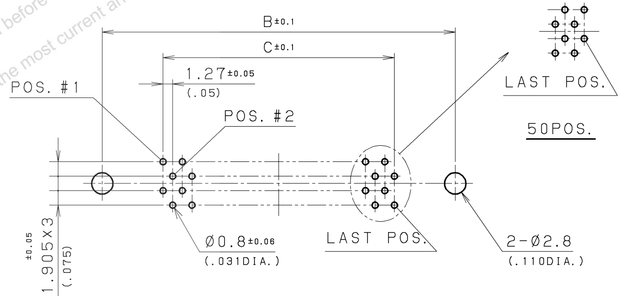
RECOMMENDED P. C. BOARD MOUNTING DIMENSIONS (CONNECTOR SIDE) P. C. BOARD THICKNESS : 1.6mm
